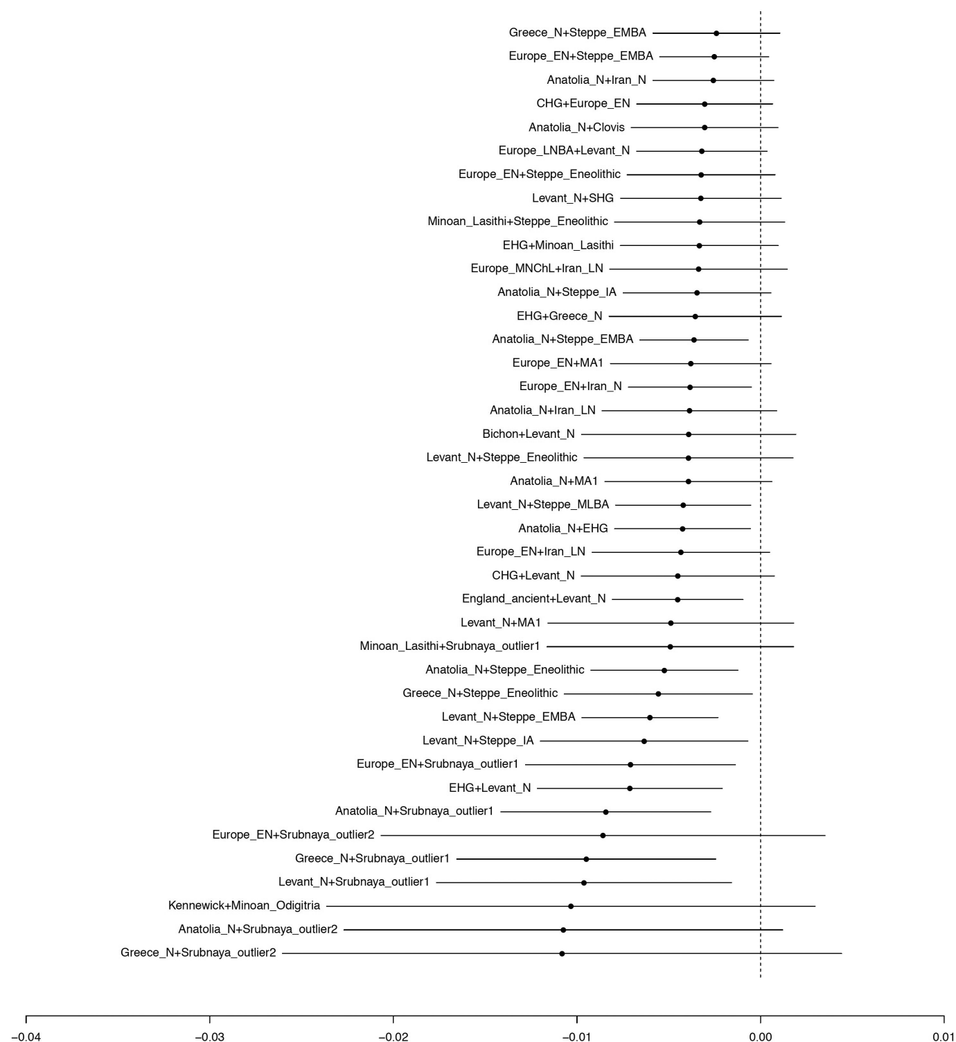
Extended Data Figure 4 | The f_3 -statistics of Mycenaeans as a target with different pairs of reference populations. The value of the statistic f_3(\text{Ref}_1, \text{Ref}_2; \text{Mycenaean}) with \pm 3 standard errors; only the population
