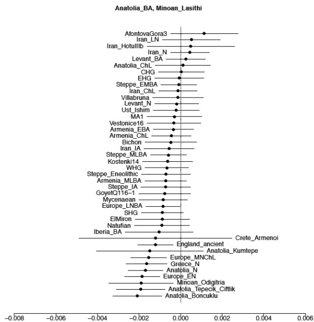
Extended Data Figure 3 | Symmetry testing of Anatolian Bronze Age populations. The statistic f_4(X, Y; \text{Test}, \text{Chimp}) is shown with \pm 3 standard errors. Each panel is titled with the pair X, Y . Populations are ordered according to the value of the statistic. Positive values indicate that Test shares more alleles with X than Y , and negative values that it shares more with Y than X . a , European, Siberian, and Caucasus hunter-gatherers share fewer alleles with Bronze Age Anatolians from Harmanören Gündürle
